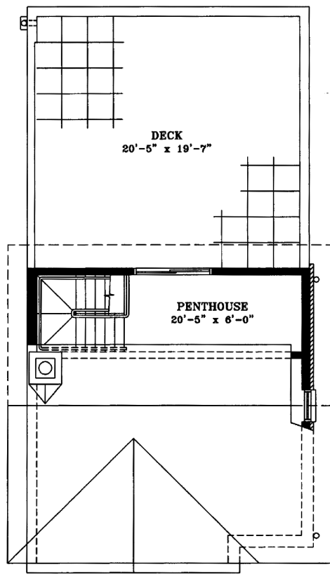
PENTHOUSE PLAN
